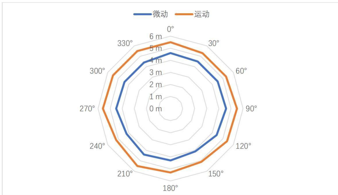
5-3 Hanging ceiling mount induction range
